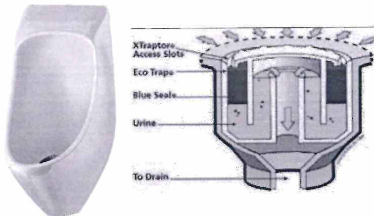
Waterless Urinal
